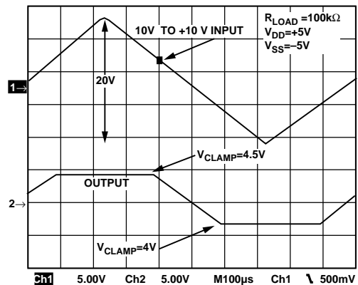
Figure 6. Overvoltage Ramp
