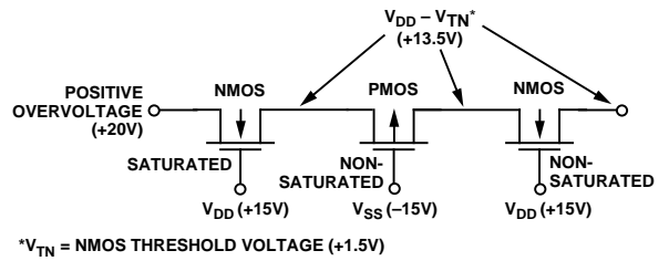
Figure 8. Positive Overvoltage on the Channel Protector
