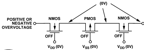
Figure 11. Channel Protector Supplies Equal to Zero Volts
