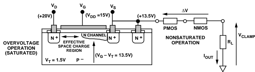
Figure 9. Positive Overvoltages Operation of the Channel Protector
