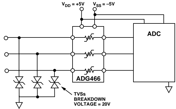
Figure 14. High Voltage Protection
