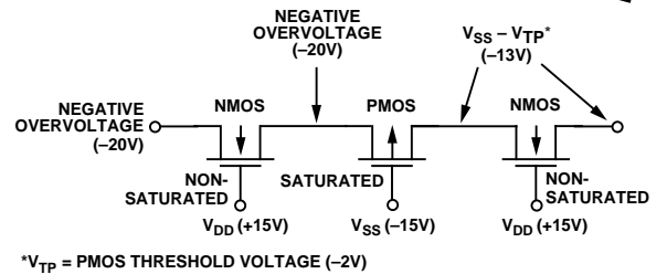
Figure 10. Negative Overvoltage on the Channel Protector
