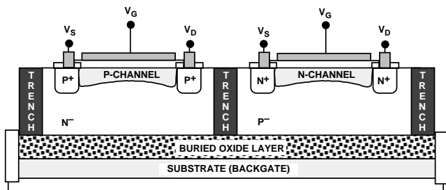
Figure 12. Trench Isolation
