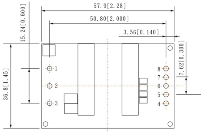
Top View (Facedown pins)
