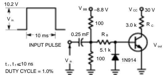
Figure 6. Switching Time Test Circuit
