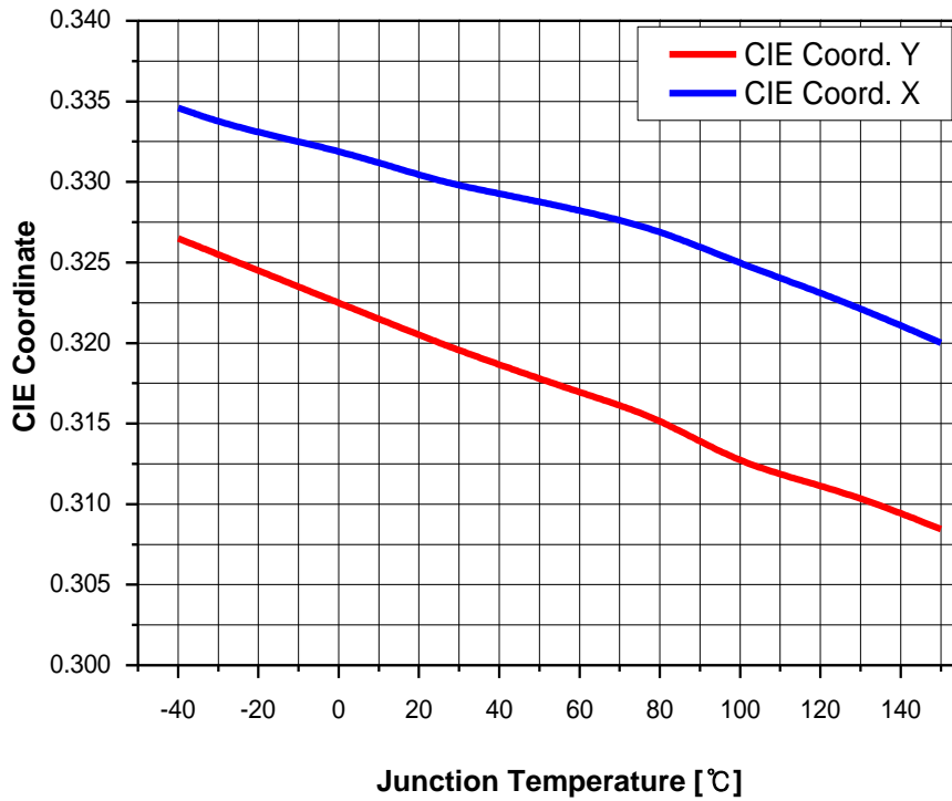
Fig 8. Chromaticity Coordinate vs. Junction Temperature, I_F = 140\text{mA}
