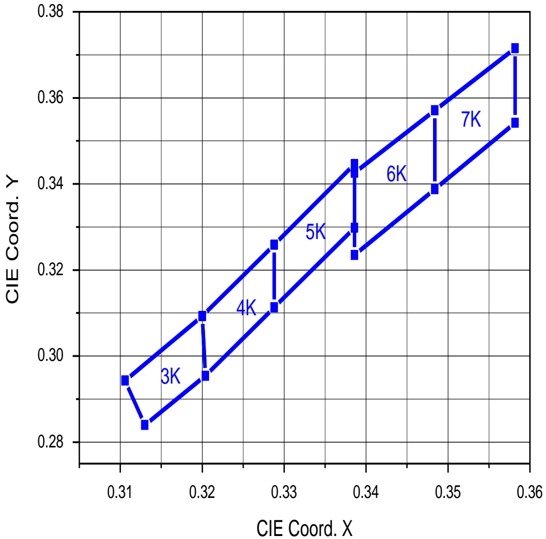
CIE Chromaticity Diagram, I_F = 140\text{mA} , T_a = 25^\circ\text{C}
