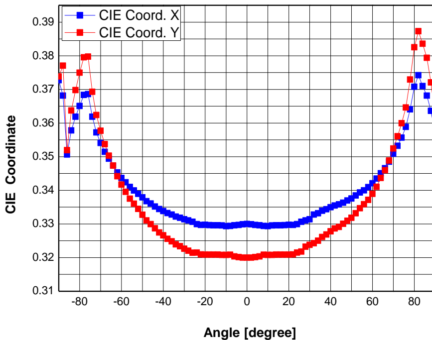
Fig 10. Color. vs. Viewing Angle, T_a = 25^\circ\text{C} , I_F=140\text{mA}
