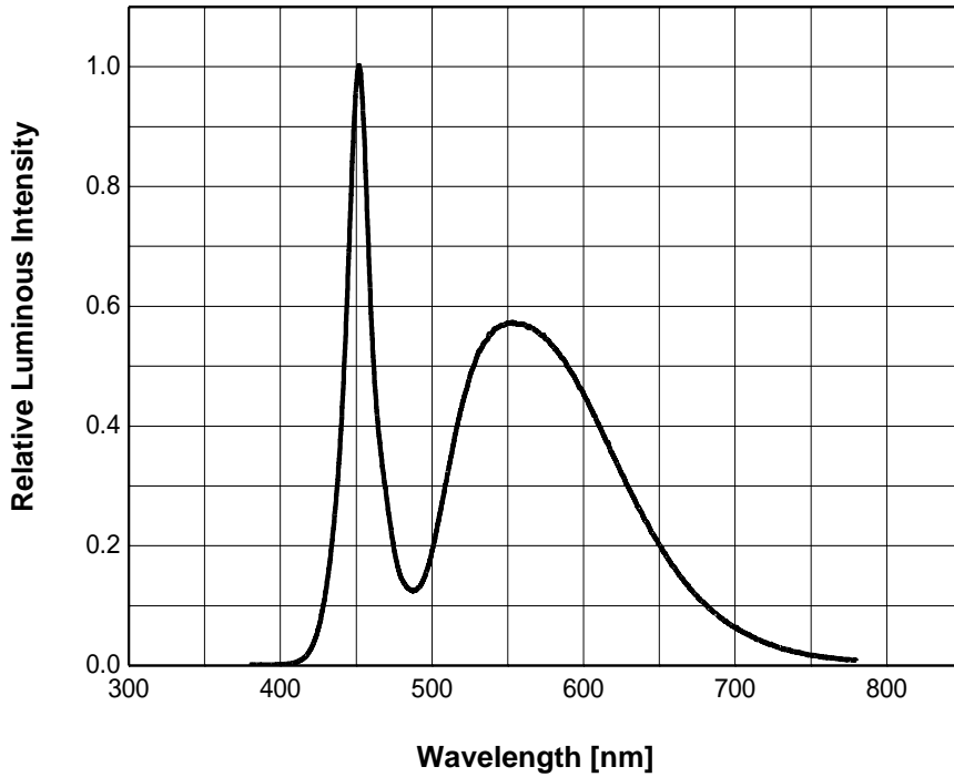
Fig 1. Color Spectrum, I_F = 140\text{mA} , T_a = 25^\circ\text{C} , RH30%
