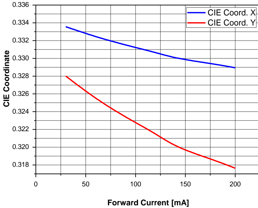
Fig 5. Forward Current vs. CIE X, Y Shift, T_a = 25^\circ\text{C}
