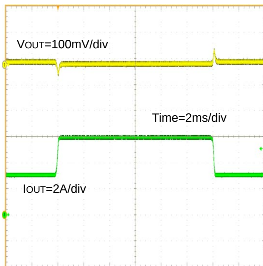
Figure 39. Load Transient Response I_{OUT} = 3A to 6A load step ( V_{IN} =5V, V_{OUT} =1.8V, L =1.5 \mu H, R_3 =6.8k \Omega , C_6 =5600pF, C_{14} =100pF)
