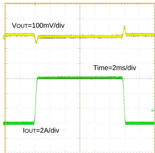
Figure 40. Load Transient Response I_{OUT} =0A to 6A load step ( V_{IN} =5V, V_{OUT} =1.8V, L =1.5 \mu H, R_3 =6.8k \Omega , C_6 =5600pF, C_{14} =100pF)
