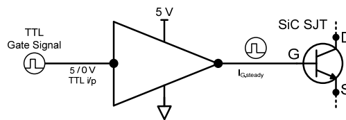
Figure 22: TTL Gate Drive Schematic
