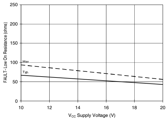
Figure 37B. FAULT Low On Resistance vs. Voltage
