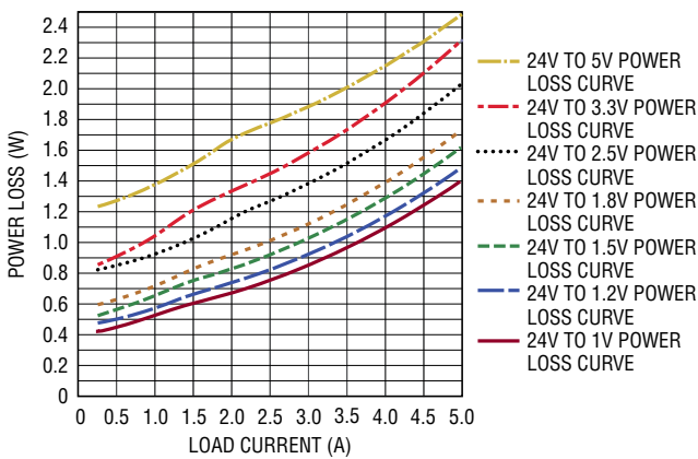
Figure 12. 24V Power Loss (Ch1 and Ch2)
