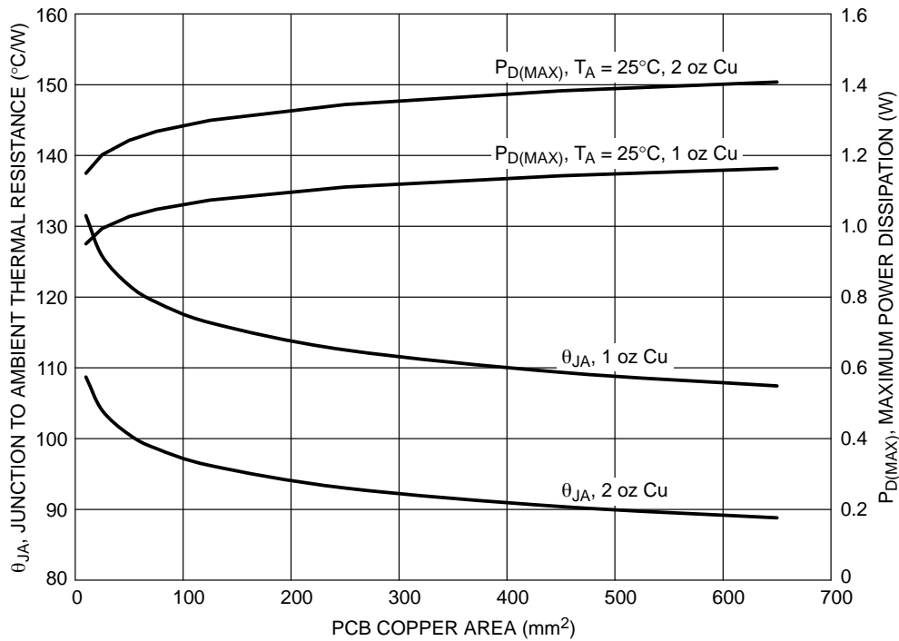
Figure 53. \theta_{JA} and P_{D(MAX)} vs. Copper Area (CSP4)
