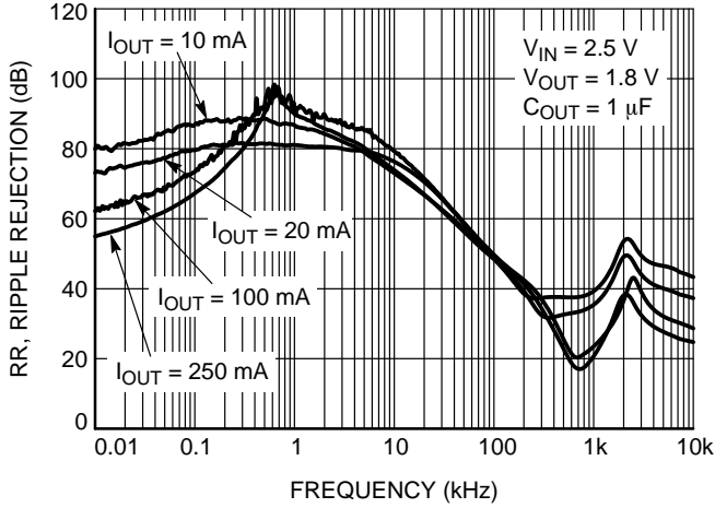
Figure 34. Power Supply Rejection Ratio, V_{OUT} = 1.8\text{ V}
