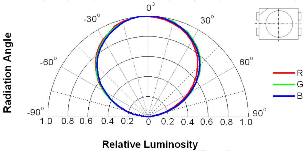
Figure5. Relative Luminosity VS. Radiation Angle
