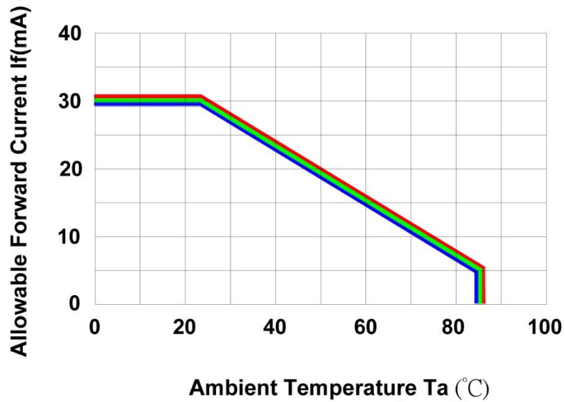
Figure 3. Ambient Temperature & forward current
