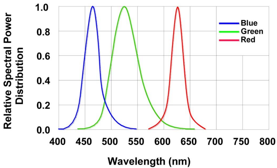
Figure 4. Relative Spectral Power Distribution vs. Wavelength
