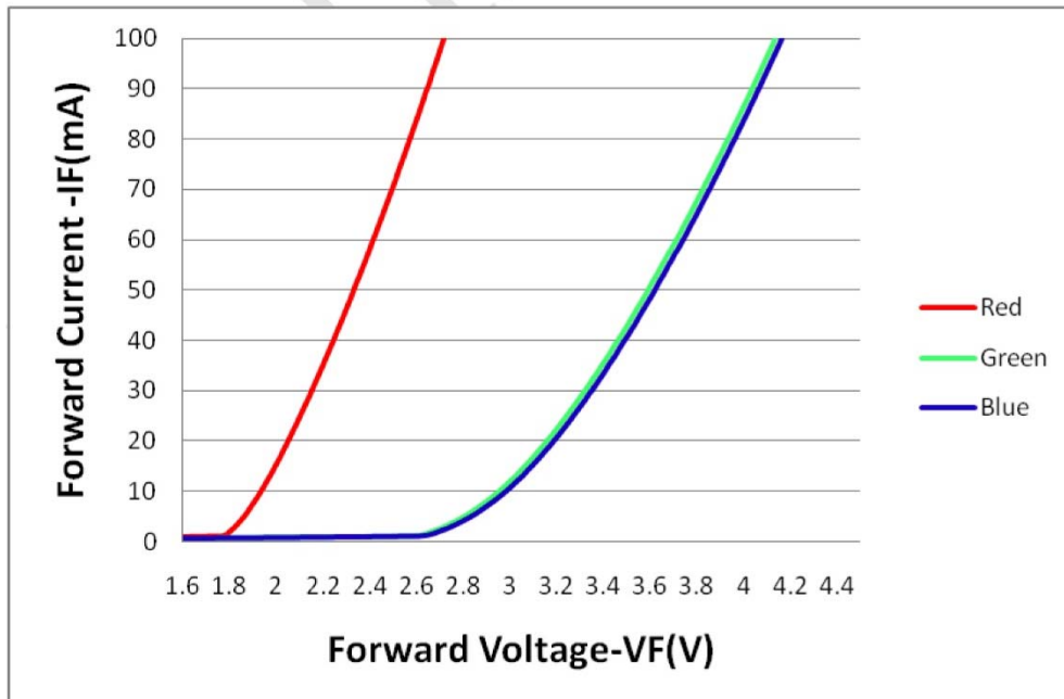
Figure2. Forward Current VS. Forward Voltage
