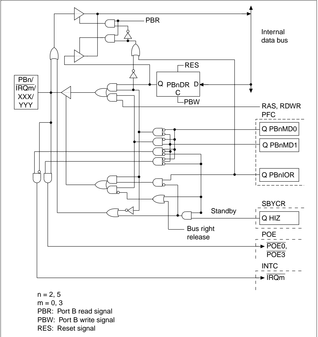
Figure B.21 PBn/\overline{IRQm}/XXXX/YYYY Block Diagram
