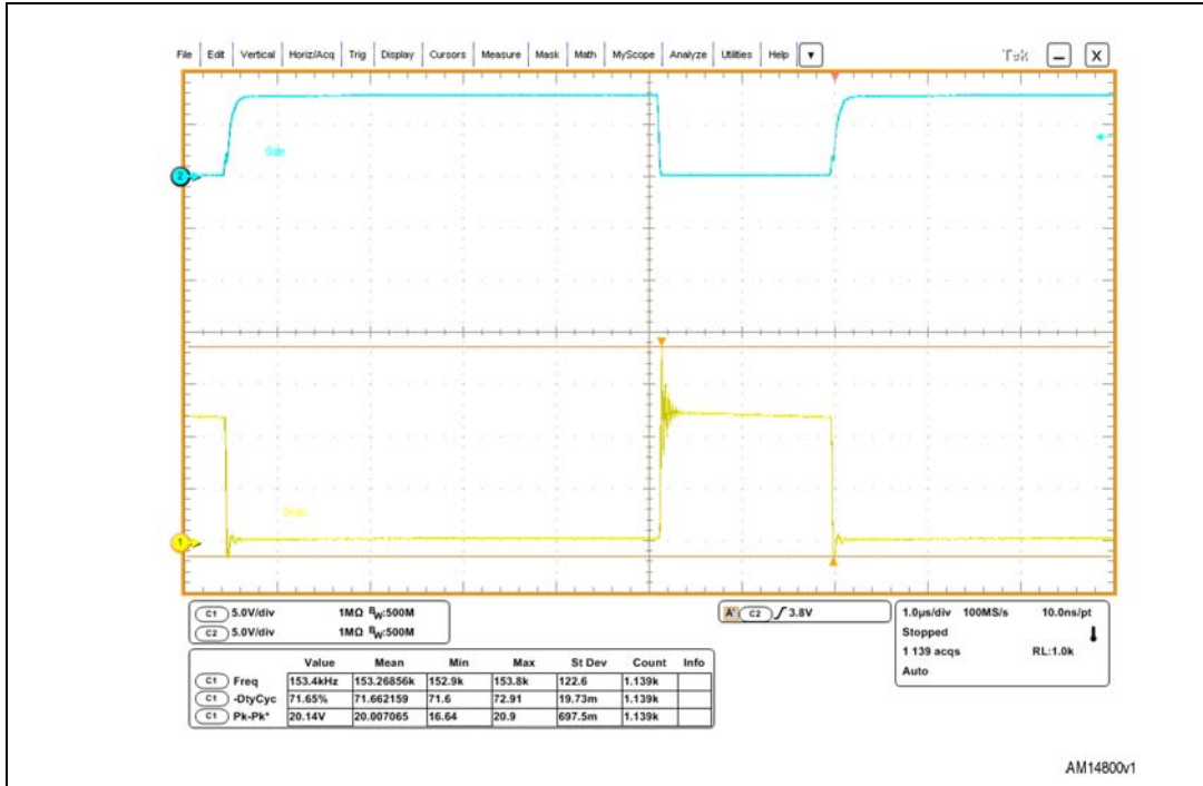
Figure 10. Secondary side Power MOSFET waveforms at 3 A load
