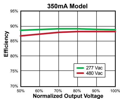
Efficiency / Load
