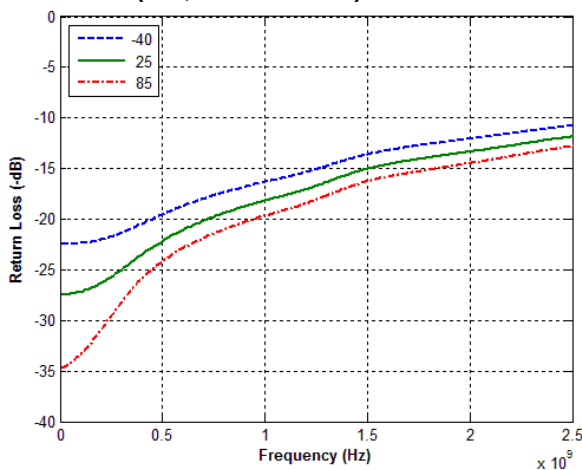
Figure 15. Return Loss vs. Temp (RX, Attenuated)
