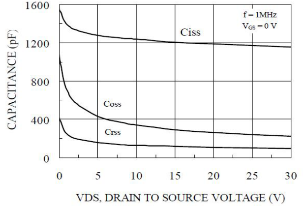
Figure 8. Capacitance Characteristics
