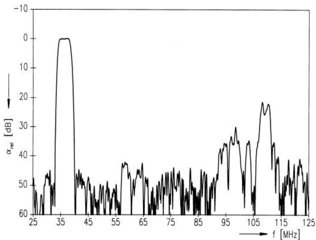
Frequency response L/L' mode (switching input pin 10 connected to input pin 1)
