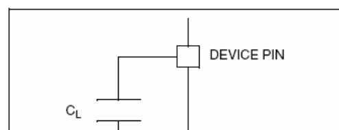
Figure 4. Pin loading conditions
