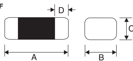
CTCB1206F
