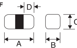
CTCB0603F
