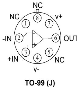
Figure 1 - Terminal connections.
