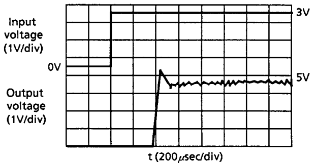
S-8321AA V_{IN} = 0 \rightarrow 3\text{V} , R_L = 250\Omega
