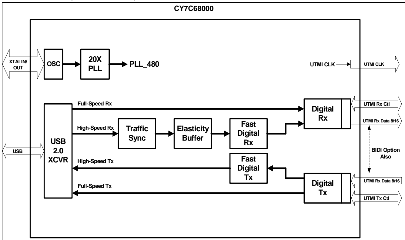
Figure 1-1. Block Diagram
