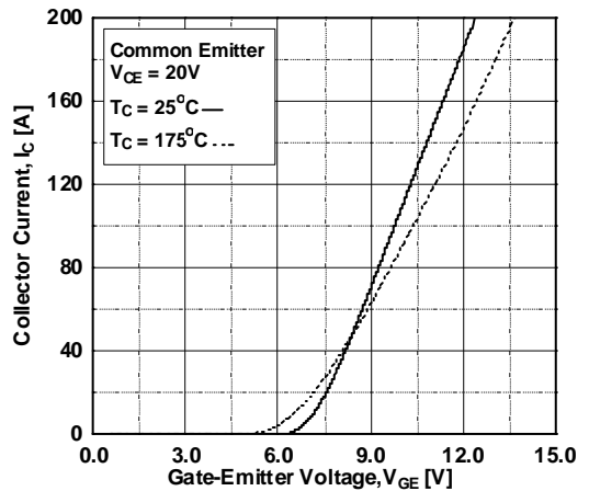
Figure 4. Transfer Characteristics
