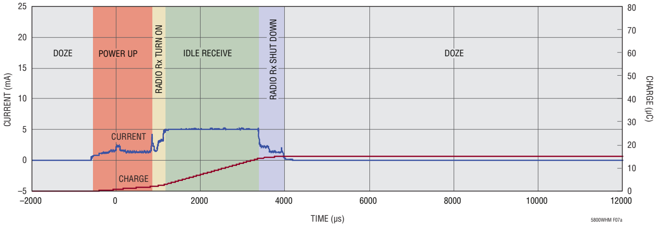
Atomic Operation – Maximum Length Transmit with Acknowledge, 10ms Time Slot (15.1 \mu C Total Charge at 3.6V)
