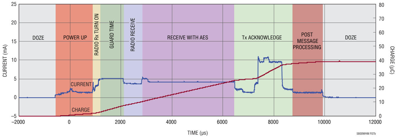
Atomic Operation – Maximum Length Transmit with Acknowledge, 10ms Time Slot (39.2 \mu C Total Charge at 3.6V)
