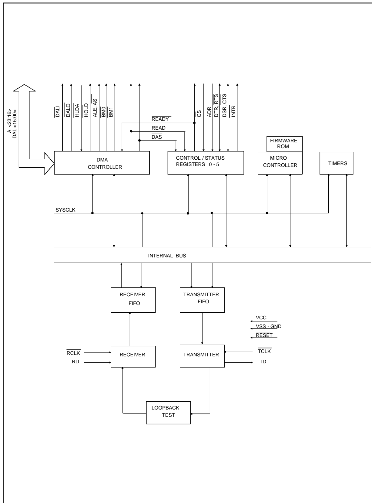
Figure 2: MK50H25 Simplified Block Diagram
