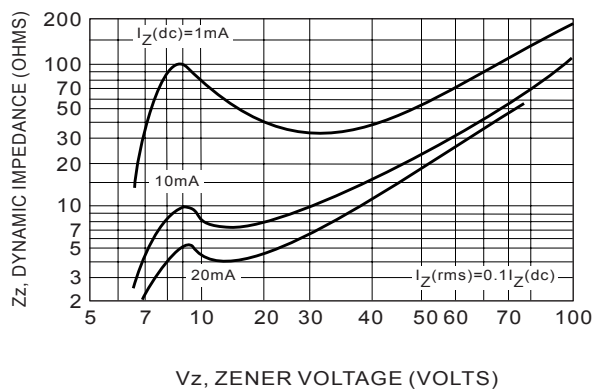
Fig.5 Effect of Zener Voltage
