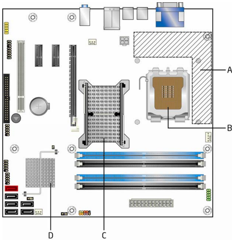
Figure 16 shows the locations of the localized high temperature zones.
