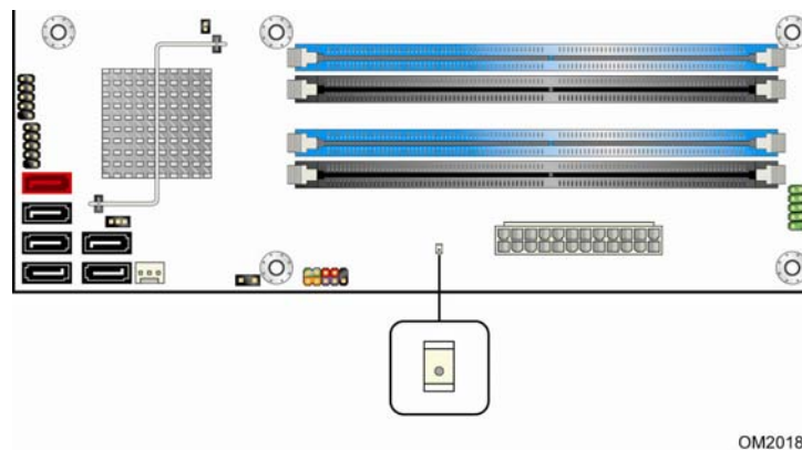
Figure 8. Location of the Standby Power Indicator LED
