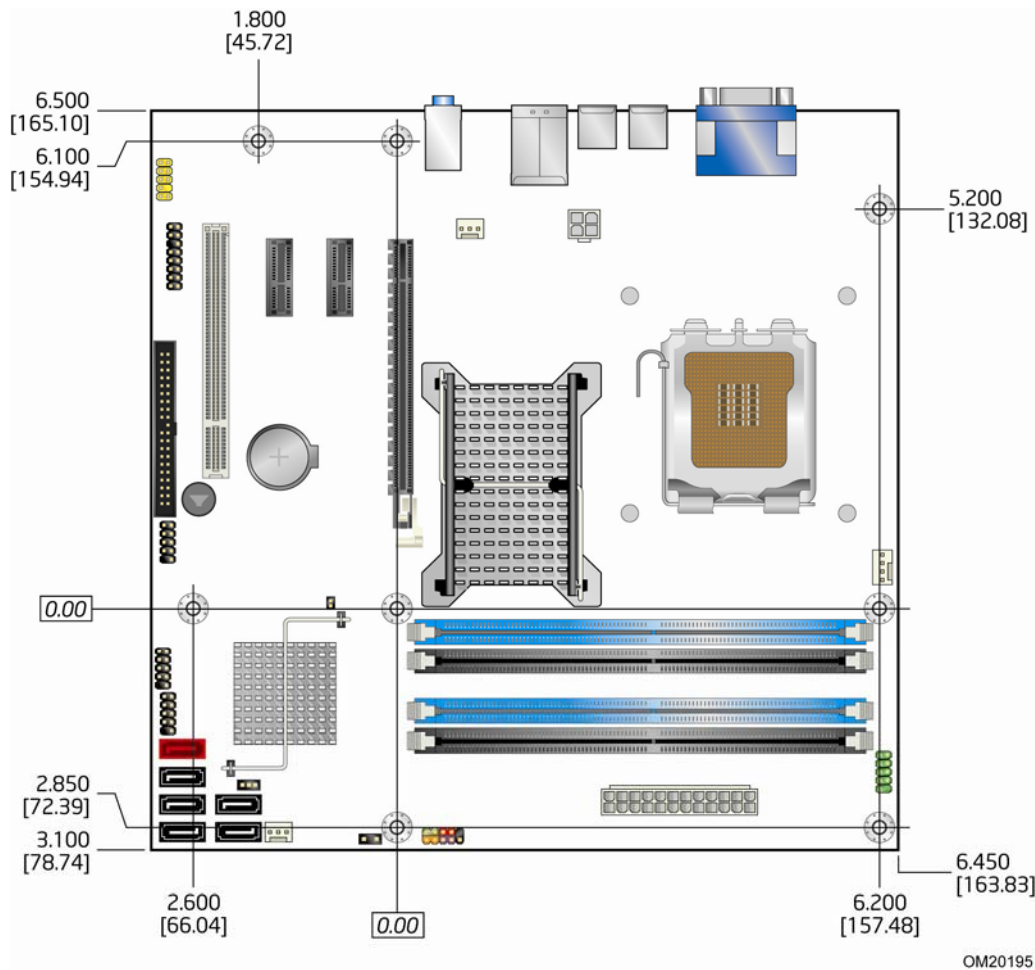
Figure 15. Board Dimensions
