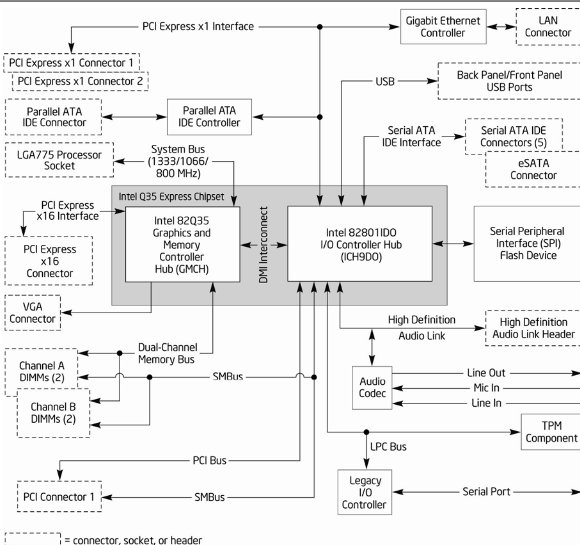
Figure 2. Block Diagram
