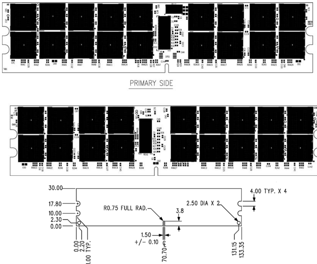
Figure 1: KVR800D2D4P6K2/8G 240-Pin DIMM
