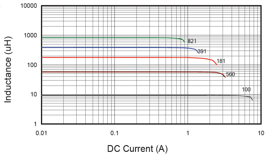
Inductance vs. DC Current
