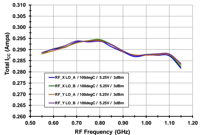
Total I CC [High Side Injection]
