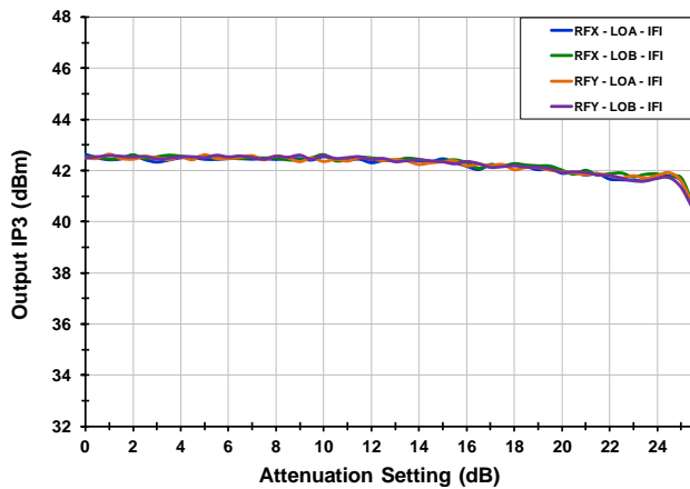
IP3 0 [0.8 GHz RF, HiSide Inj.]
