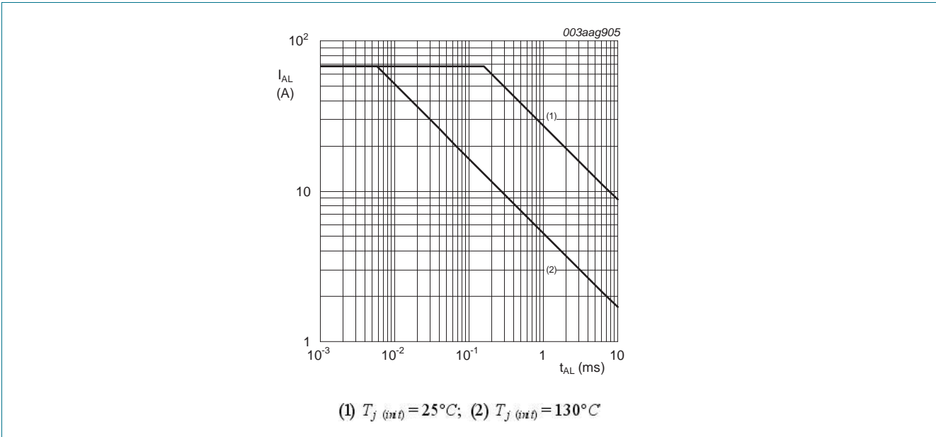
Fig 3. Single pulse avalanche rating; avalanche current as a function of avalanche time
