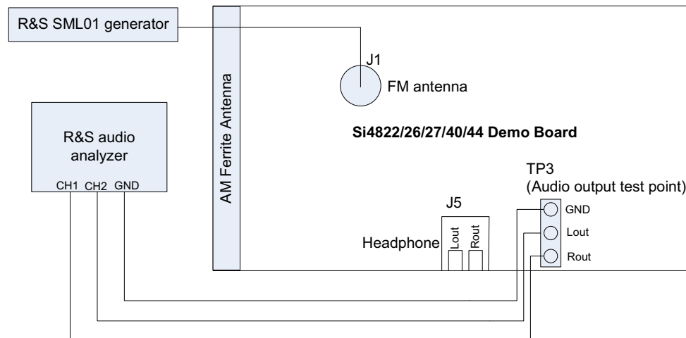
Figure 1. FM Tuner Setup with One Generator
