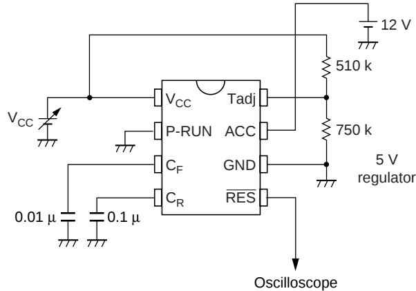
Test circuit
