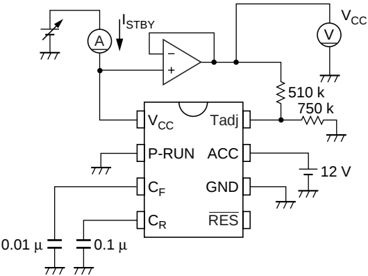
Test circuit
