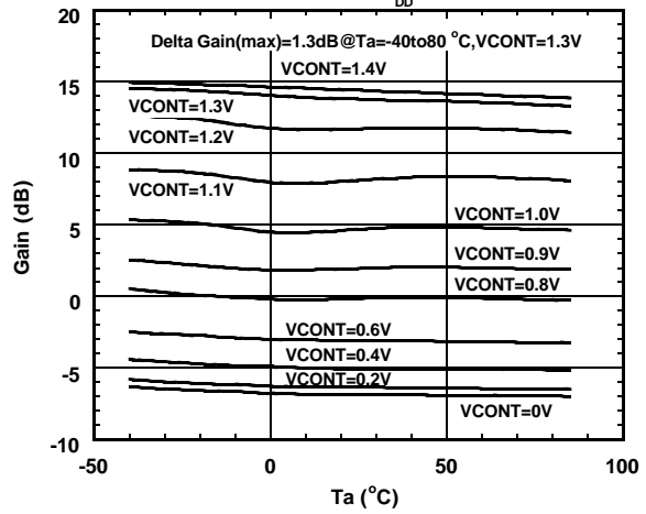
Gain vs. Ta (Variable VCONT)
