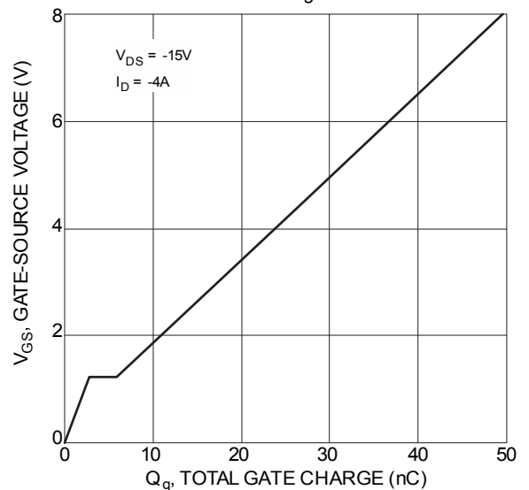
Figure 12 Gate-Charge Characteristics
