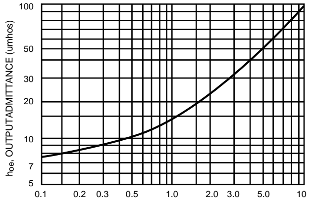
Figure 10. Output Admittance
