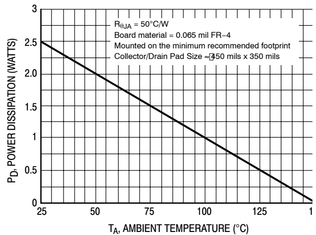
Figure 15. D 2 PAK Power Derating Curve
