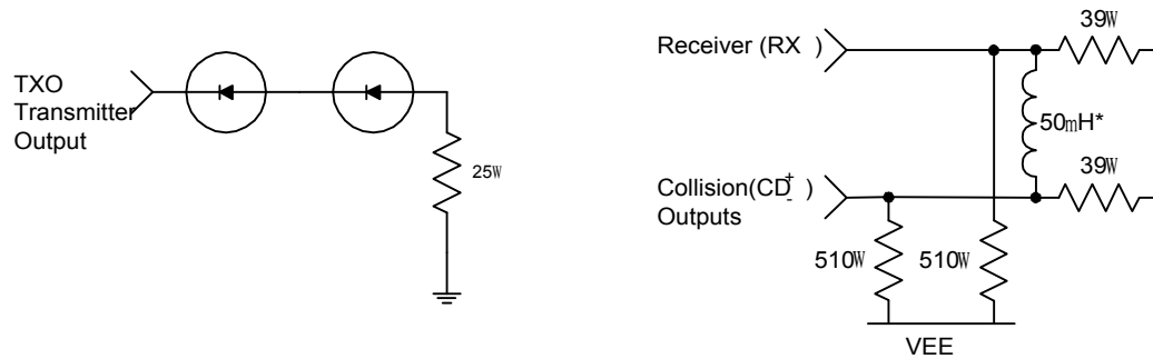
Figure 6. Test Loads
