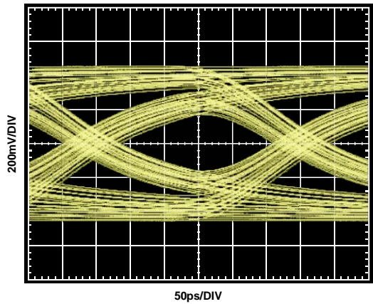
Figure 10. 3.25 Gbps Input Eye, 30 Inch FR4 Input Channel (TP2 from Figure 9)
