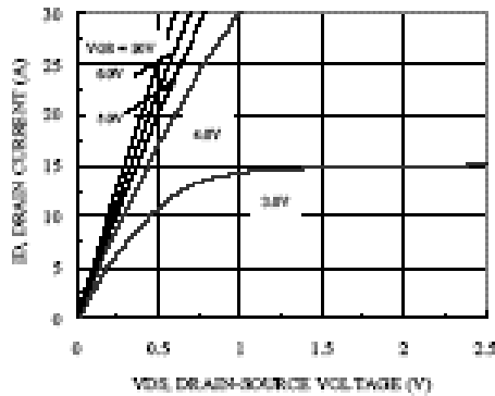
Figure 1. On-Region Characteristic
