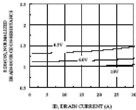
Figure 3. On Resistance vs V_{GS} Voltage
