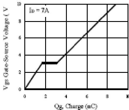
Figure 5. Gate Charge Characteristic
