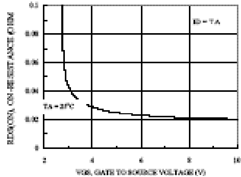
Figure 8. On-Resistance with Gate to Source Voltage
