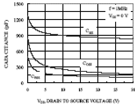
Figure 4. Capacitance Characteristics
