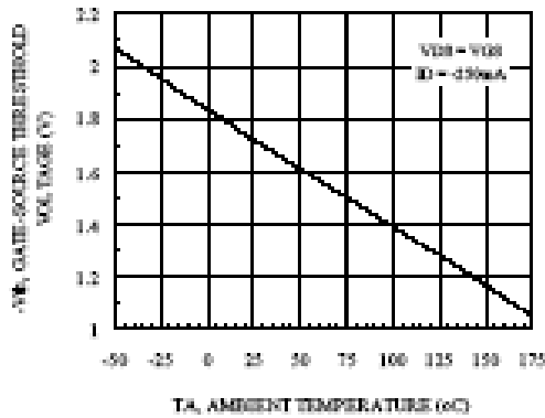
Figure 9. V GS Gate to Source Voltage V GS Temperature
