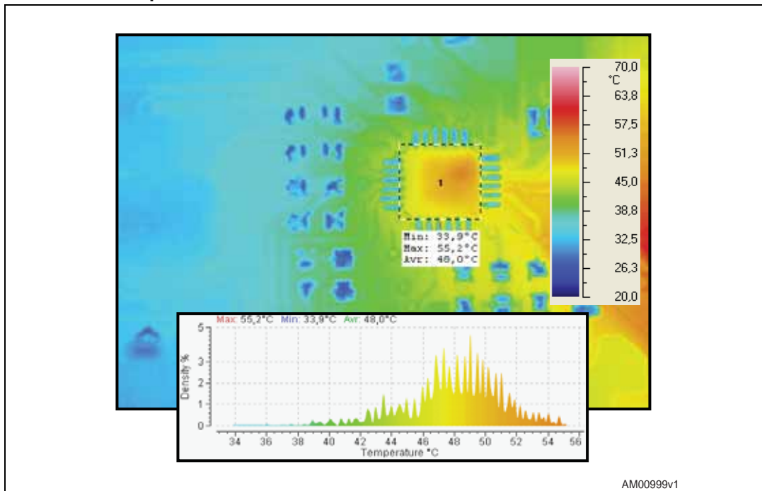
Figure 38. I_{LOUT} = 1.0\text{ A} , average IC temperature = 48^{\circ}\text{C} , max internal IC temperature = 55.2\text{ }^{\circ}\text{C}
