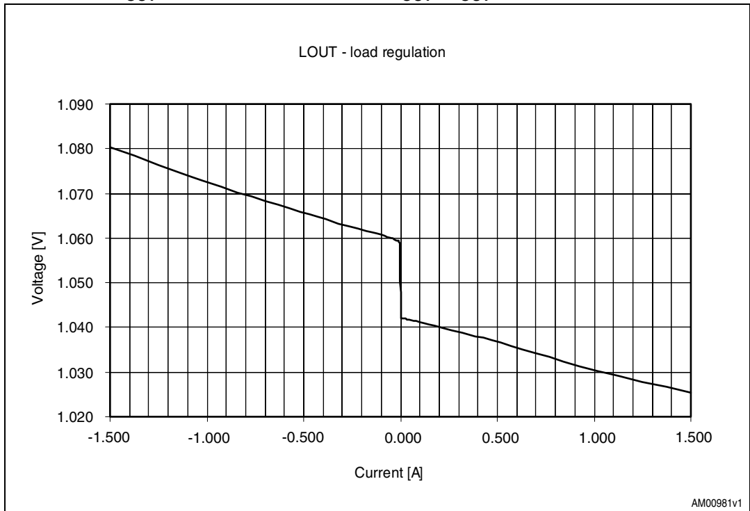
Figure 20. L_{OUT} load regulation - LDOIN = V_{OUT} , V_{OUT} in forced PWM mode
