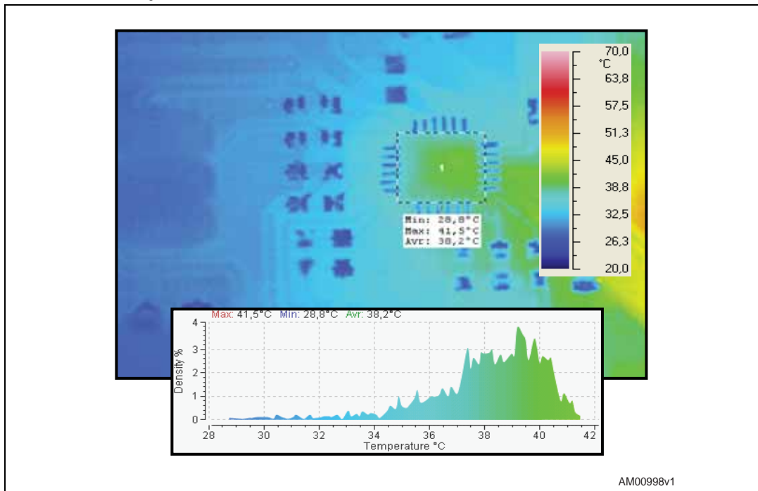
Figure 37. I_{LOUT} = 0.5\text{ A} , average IC temperature = 38.2\text{ }^{\circ}\text{C} , max internal IC temperature = 41.5\text{ }^{\circ}\text{C}
