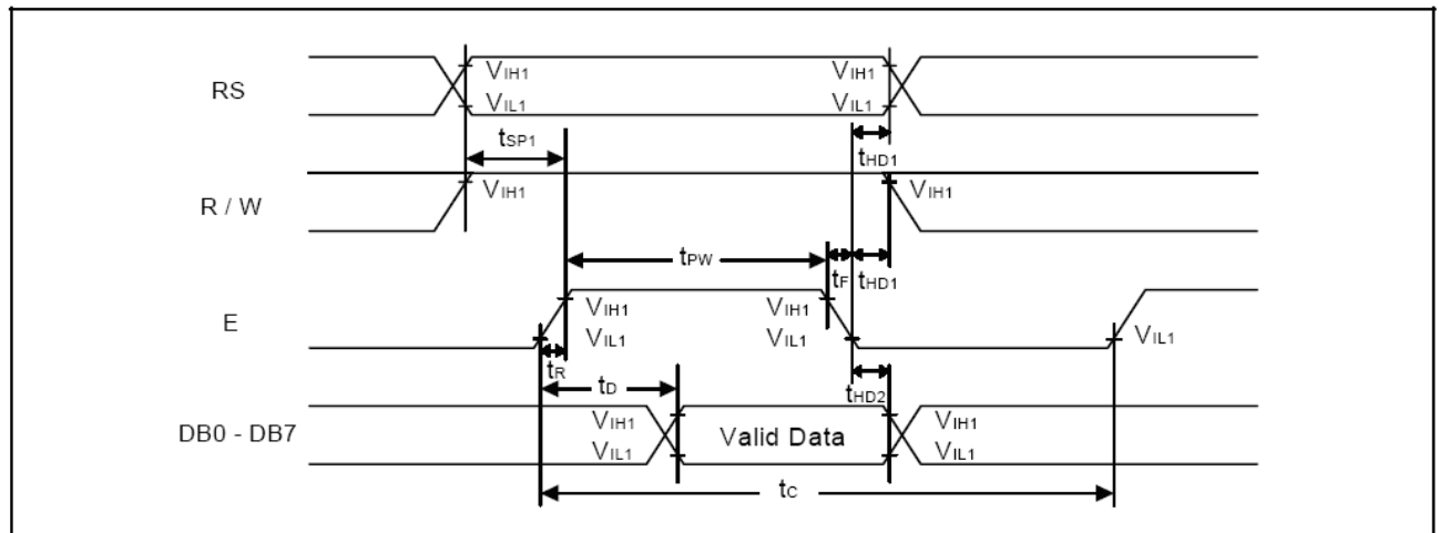
Read mode timing diagram (Reading Data from SPLC780C to MPU)
