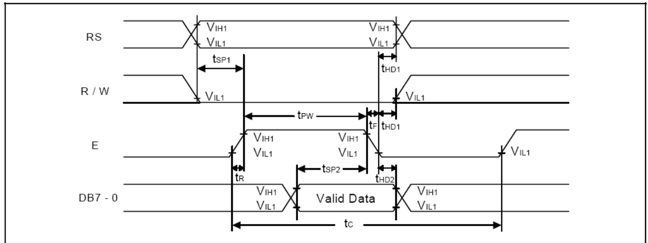
Write mode timing diagram (Writing Data from MPU to SPLC780C)
