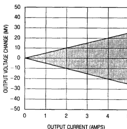
Load Regulation *
