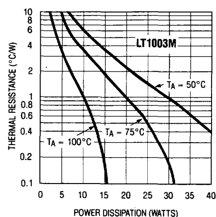
Suggested Heat Sink Thermal Resistance (LT1003M)
