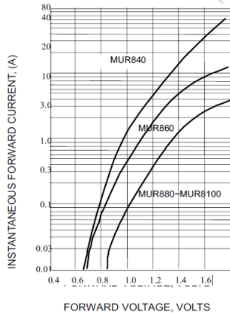
Fig. 4-TYPICAL FORWARD CURRENT
