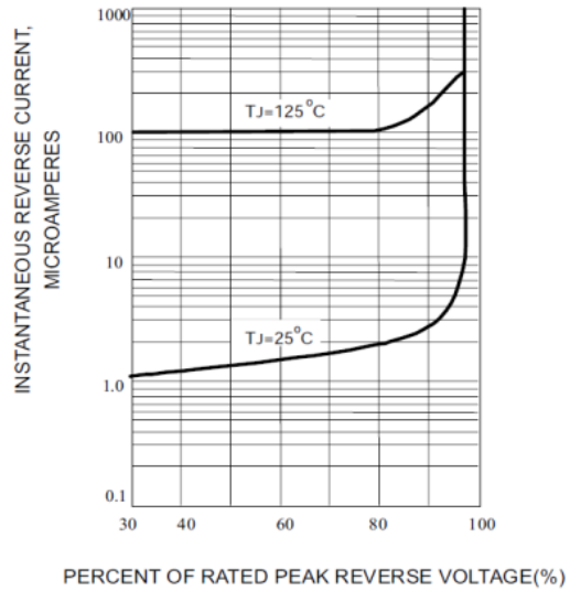
Fig. 2-TYPICAL REVERSE CHARACTERISTICS
