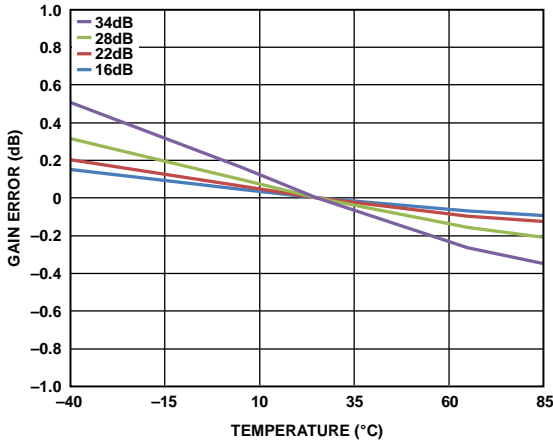
Figure 5. Gain Error vs. Temperature at All Gains
