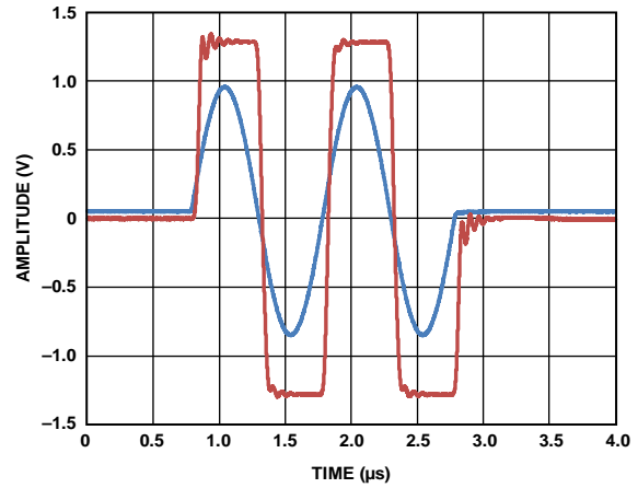
Figure 19. Overdrive Recovery
