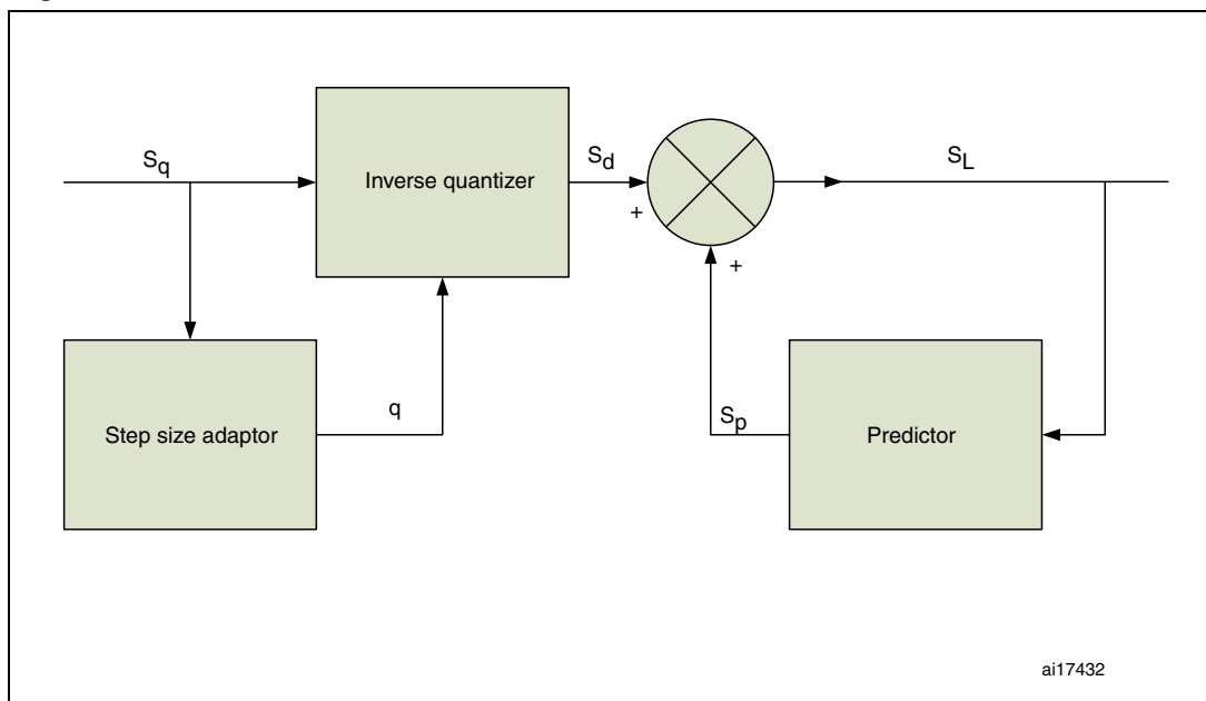
Figure 1. ADPCM decoder
