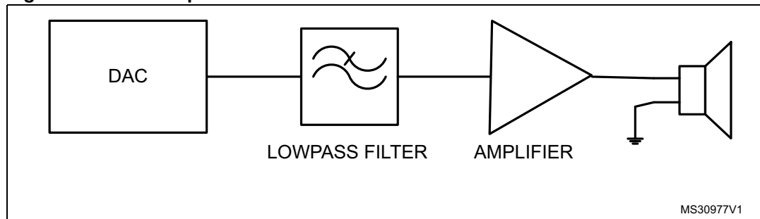
Figure 4. DAC output
