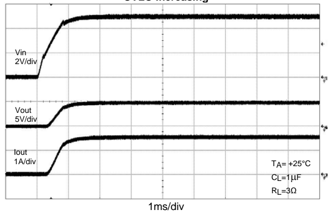
UVLO Increasing
