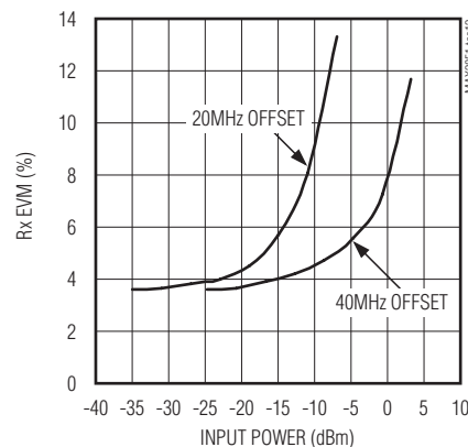
Rx EVM vs. OFDM JAMMER POWER AT 20MHz AND 40MHz OFFSET FREQUENCY WITH WANTED SIGNAL AT -66dBm
