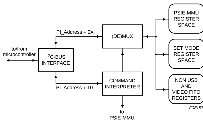
Fig.23 I 2 C-bus interface and register map.
