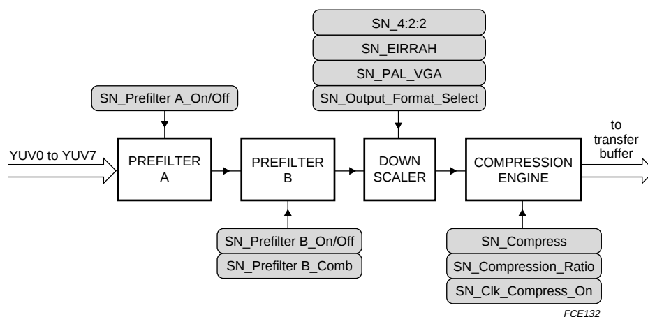
Fig.3 The CIF formatter and compression engine.
