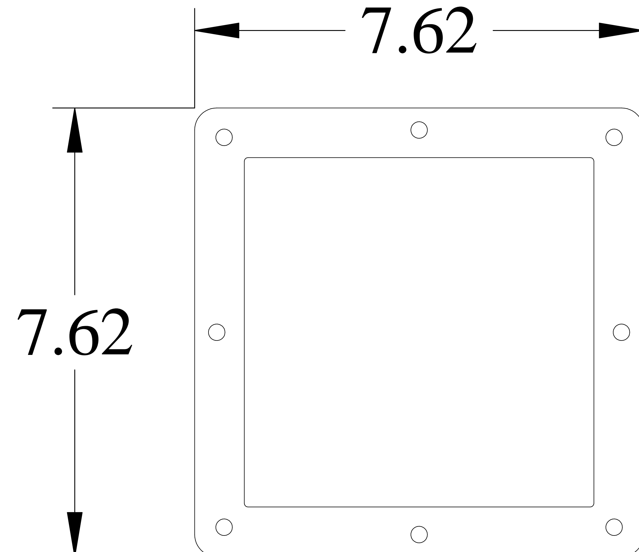
FRONT VIEW
