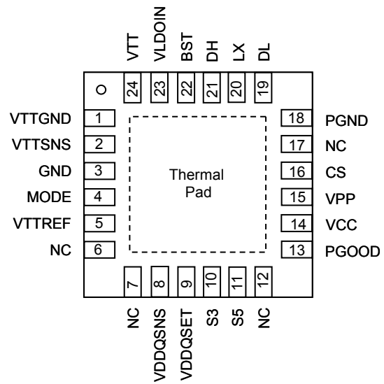
G5616 TQFN4X4-24
