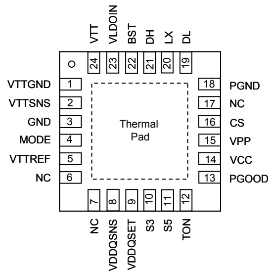
G5616A TQFN4X4-24
