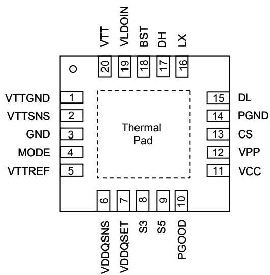
G5616 TQFN3X3-20
