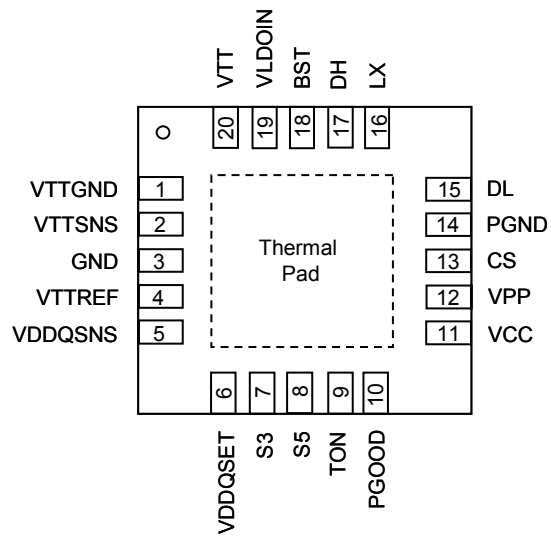
G5616A TQFN3X3-20
